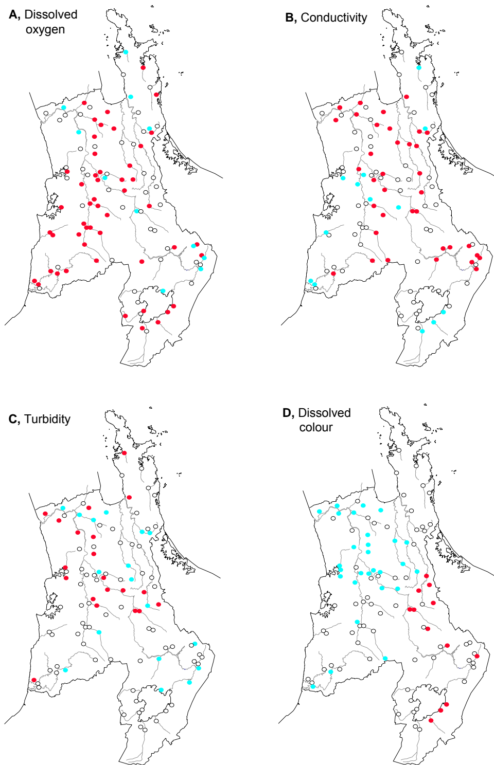
Figure 5: Nature of trends for selected water quality variables at regional river sites during 1990–2007: sites showing improving trends are shown in blue, those showing deteriorating trends in red, and those showing no significant trends as open circles. A, Dissolved oxygen; B, conductivity; C, turbidity; D, dissolved colour; E, total nitrogen; F, ammonia; G, total phosphorus; and H, dissolved reactive phosphorus. See Figure 1 and Table 5 for details; and see text for a discussion of the direction of the trends in dissolved colour.
