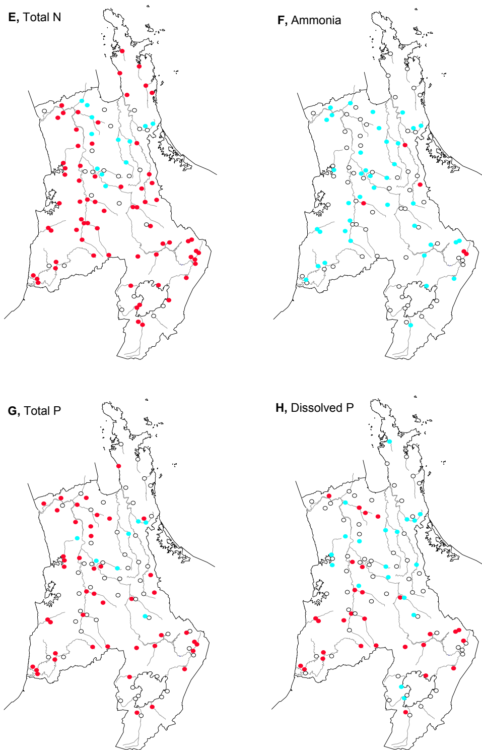
Figure 5 (continued): Nature of trends for selected water quality variables at regional river sites during 1990–2007: sites showing improving trends are shown in blue, those showing deteriorating trends in red, and those showing no significant trends as open circles. A , Dissolved oxygen; B , conductivity; C , turbidity; D , dissolved colour; E , total nitrogen; F , ammonia; G , total phosphorus; and H , dissolved reactive phosphorus. See Figure 1 and Table 5 for details; and see text for a discussion of the direction of the trends in dissolved colour.
