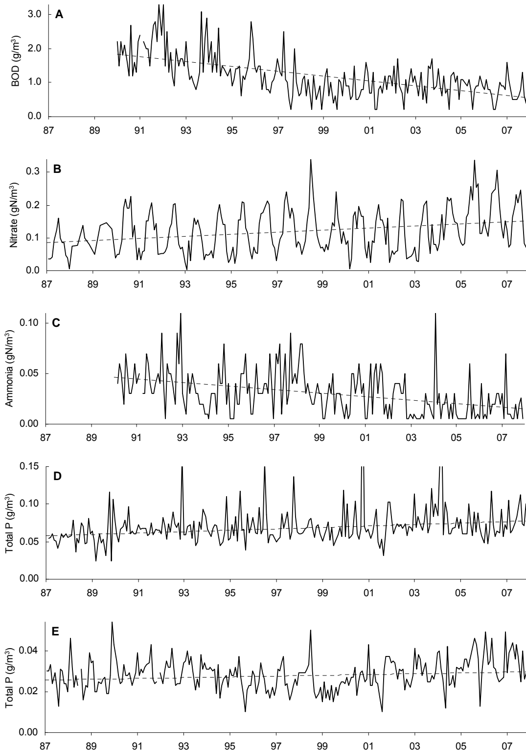
Figure 2: Water quality at Waikato River sites during 1987–2007: A, BOD 5 at Horotiu (site G); B, nitrate at Waipapa (site E); C, ammonia at Horotiu (site G); D, total phosphorus at Mercer (site I); and E, total phosphorus at Waipapa (site E). The dashed lines show the overall trends in the records.
