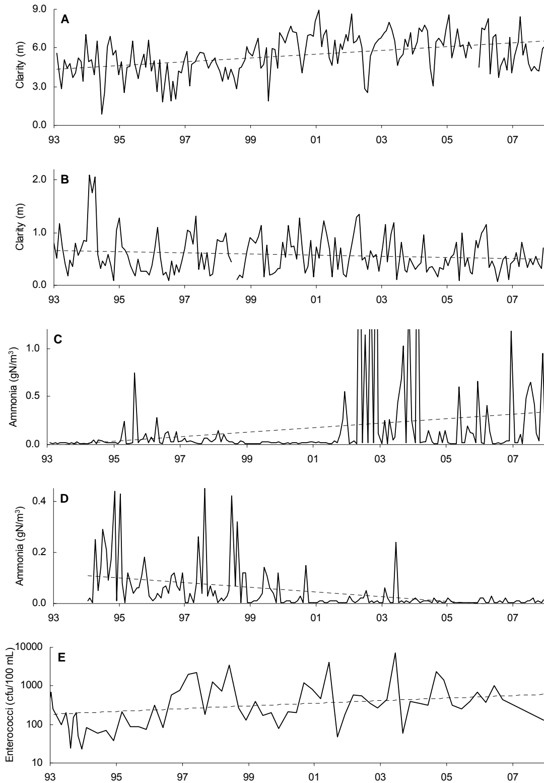
Figure 3: Water quality at various sites during 1993–2007: A, Visual clarity at Waihou (Whites, #37); B, visual clarity at Waipa (Whatawhata, #1); C, ammonia at Kawaunui (#48); D, ammonia at Mangaonua (Te Miro, #84); and E, enterococci (logarithmic) at Piako (Paeroa-Tahuna, #79). The dashed lines show the overall trends in the records.
