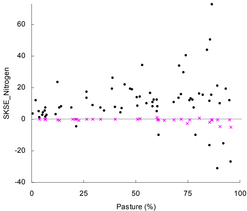
Figure 7: Trend slopes (SKSE, units as in Table 5) and land use (as percent of catchment in pasture) for total nitrogen (circles) and ammonia (crosses): redrawn from Figures 6B and 6C, respectively.
