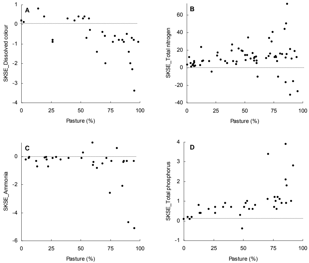
Figure 6: Slopes for significant trends (SKSE, units as in Table 5) and land use (as percent of catchment in pasture) for selected water quality variables: A, Dissolved colour; B, total nitrogen; C, ammonia; and D, total phosphorus (excluding three outliers: see text).
