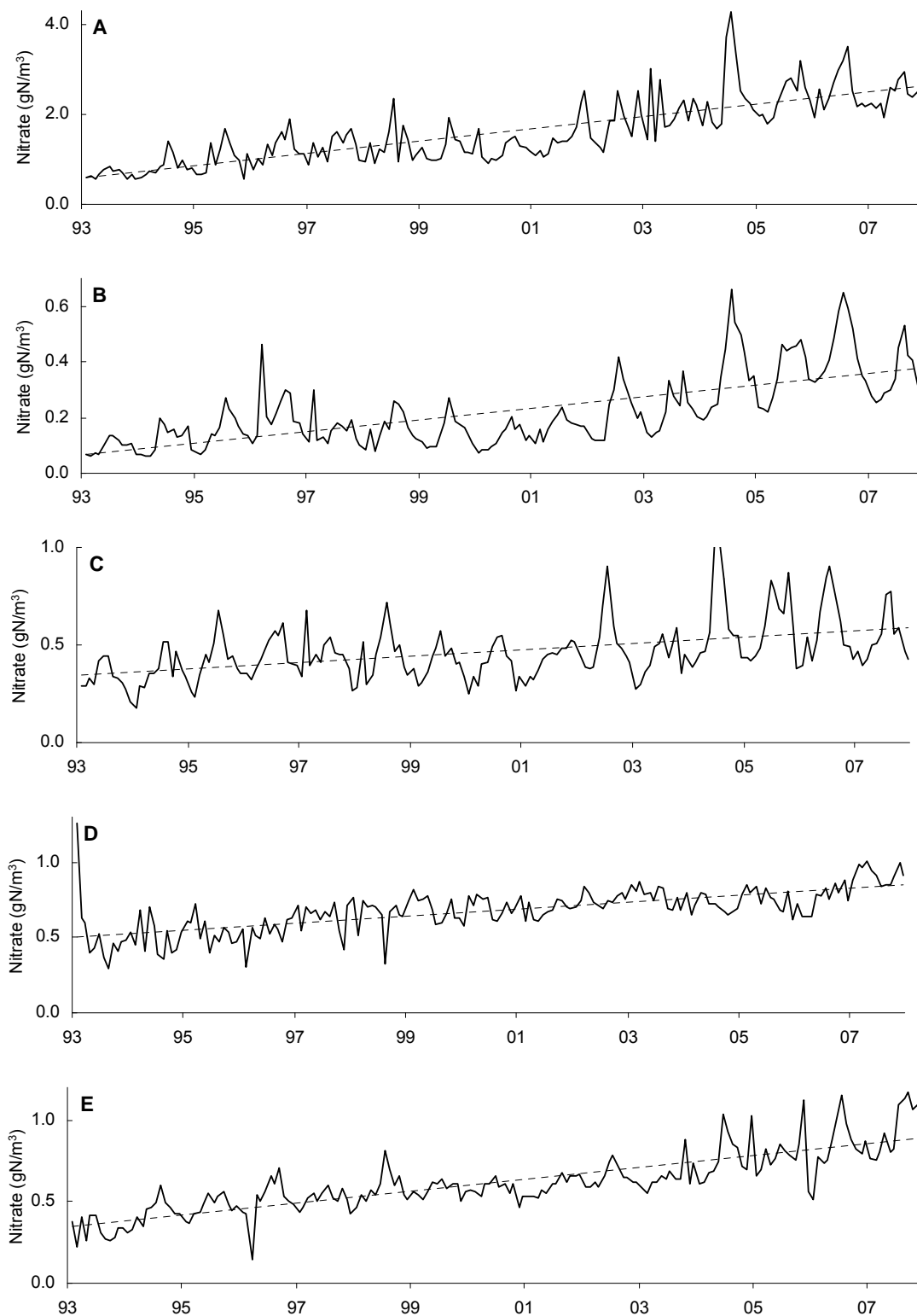
Figure 4: Nitrate concentrations at various sites in the Upland Waikato zone during 1993–2007. A, Kawaunui (#48); B, Mangaharakeke (#43); C, Tahunaatara (#44); D, Waiotapu (Campbell, #47); and E, Waipapa (#42). The dashed lines show the overall trends in the records.
